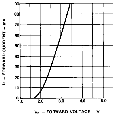
Figure 17. Forward Current vs. Forward Voltage.
