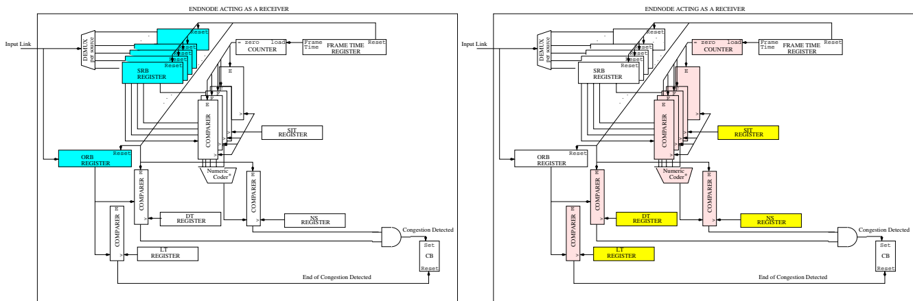
Figure 1. Logic for measuring congestion and detecting congestion.
