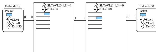
Figure 2. Example of the VLs used in IBA.
