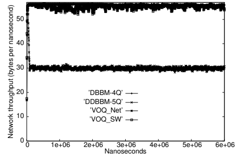
Figure 3. Accepted traffic. SIT = 0
