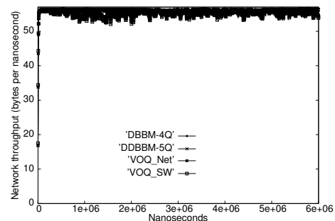
Figure 4. Accepted traffic. SIT = 6
